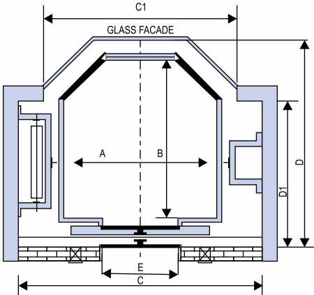
HOIST WAY PLAN FOR CAPSULE LIFT
