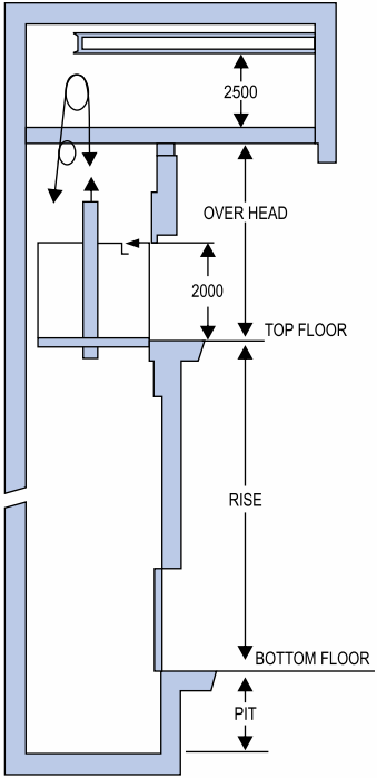
HOIST WAY PLAN FOR FREIGHT ELEVATOR
