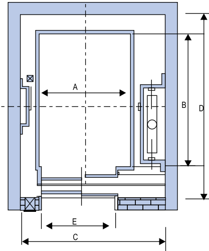
HOIST WAY PLAN FOR HOSPITAL ELEVATOR
