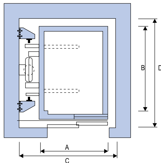
HOIST WAY PLAN FOR HYDRAULIC ELEVATOR
